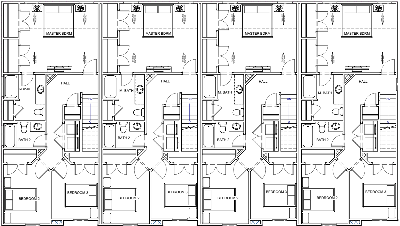
SECOND FLOOR
